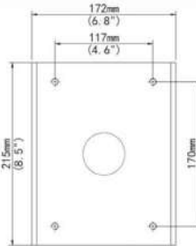
EC-UP08PM
